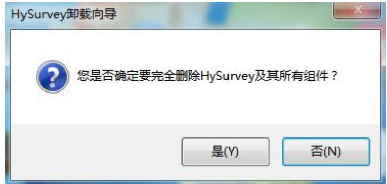
图 1-9 卸载向导
